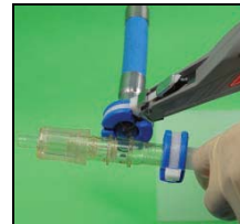
Finish closure by using SaniSure clamp tool to calibrated tension
