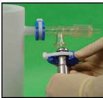
Position SaniSure Clamp around tri-clamp fitting
